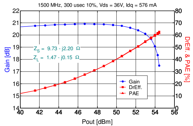
T1G2028536-FL Gain DrEff. and PAE vs. Pout
